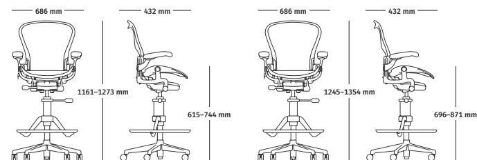
Stool with Low Cylinder
