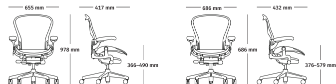
Work Chair Size A
